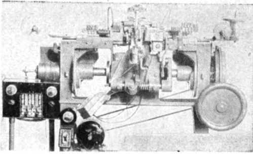
Automatic lead-in wire-welding machine made in 1919 by Bruckner of Germany. Eisler installed the machine for Save Electric Co. in 1920.
